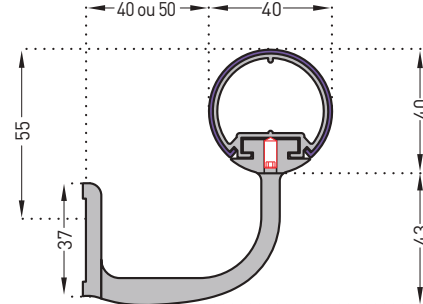
55 mm bugled self-locking aluminium bracket silver anodised effect (overall projection 80 mm or 90 mm on request)
