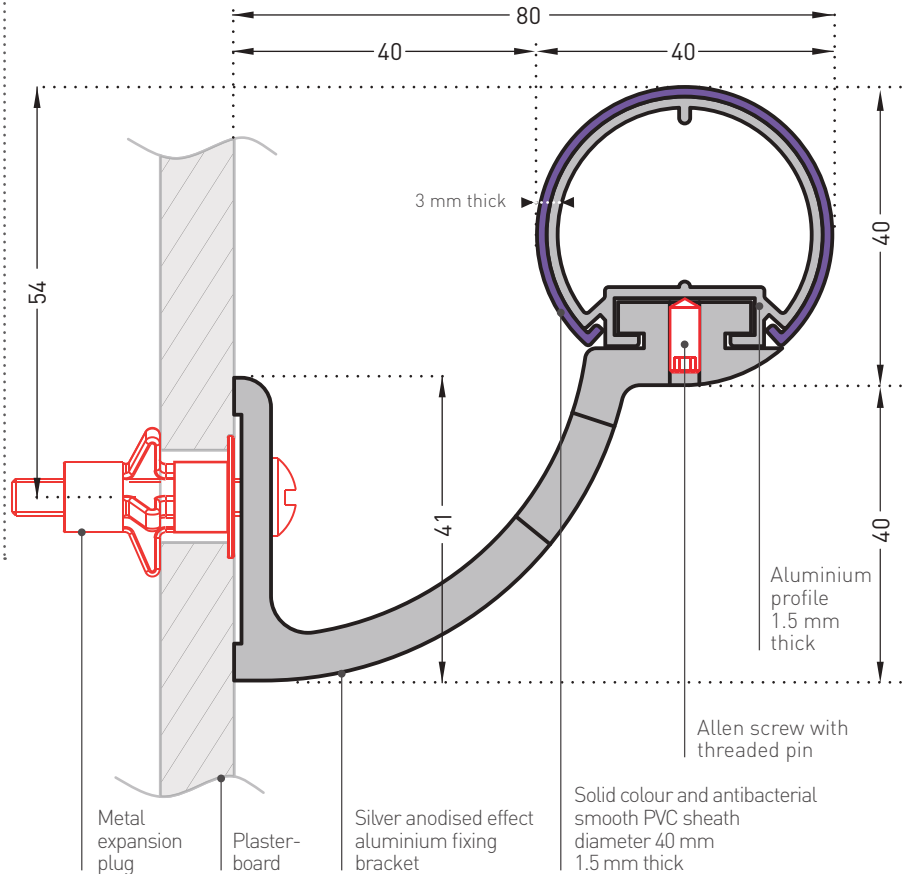
80 mm perforated self-locking aluminium bracket silver anodised effect (overall projection 80 mm)
