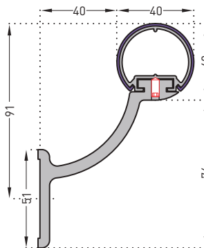
60 mm full self-locking aluminium bracket silver anodised effect (overall projection 80 mm)
