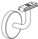
Swan-neck with 70 mm rose self-locking brushed stainless steel bracket (overall projection 80 mm)
